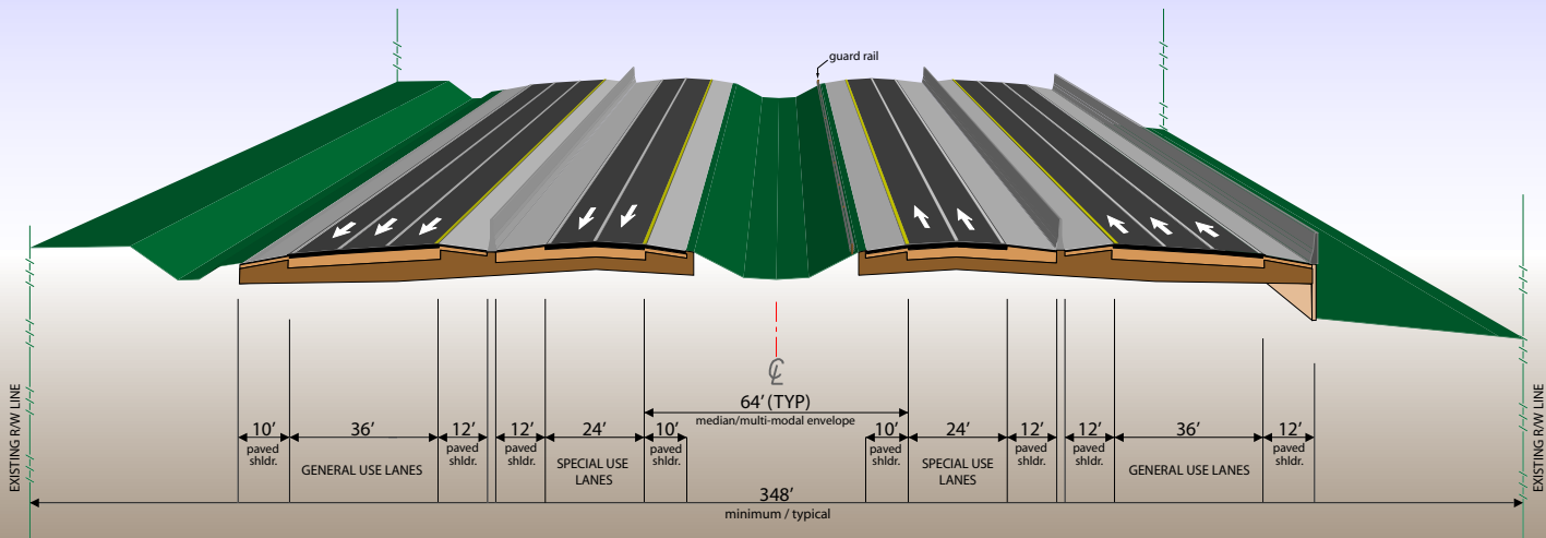
10-LANE (6 + 4 LANES) ULTIMATE TYPICAL SECTION
